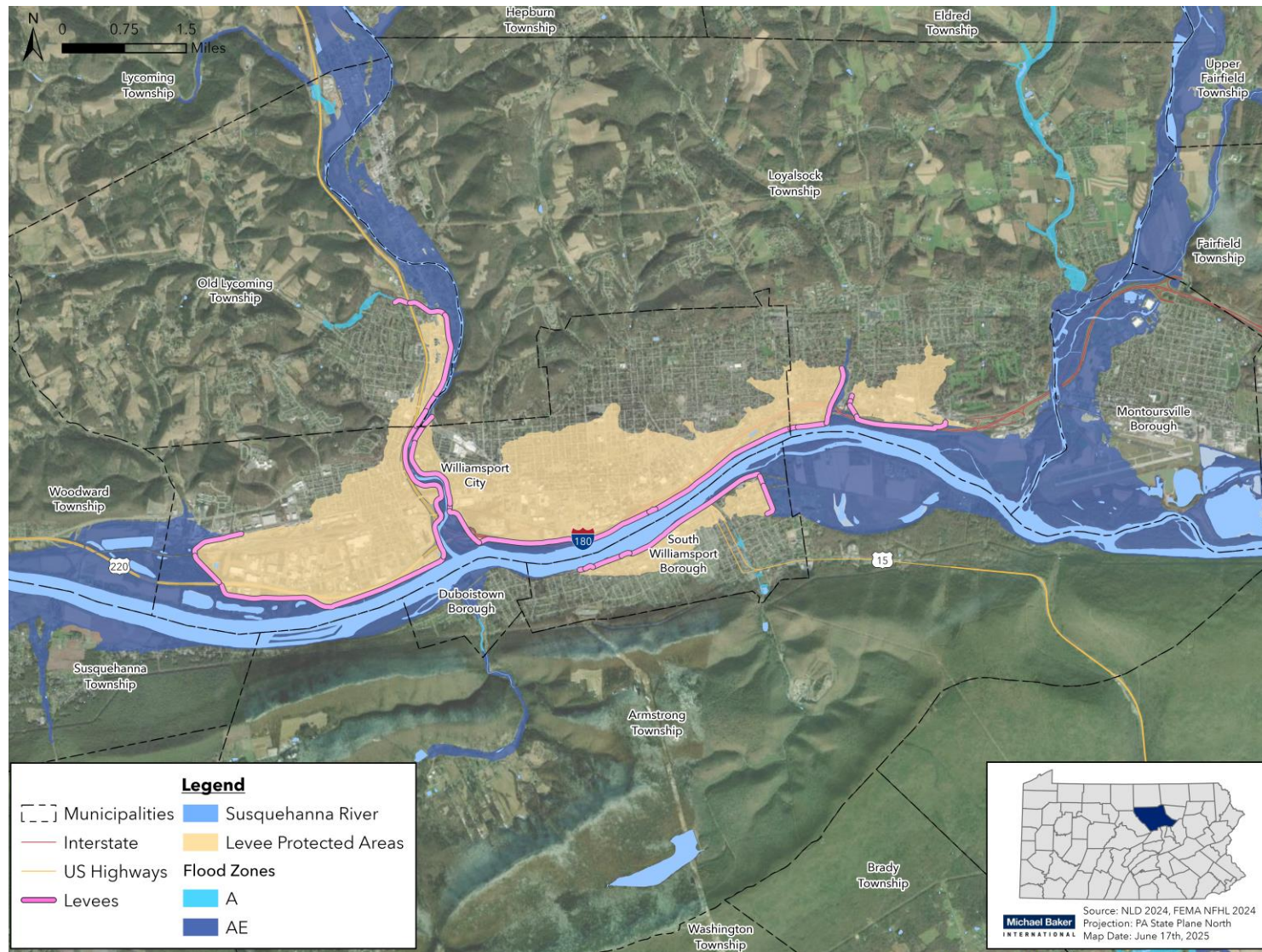
Figure 4.3.20-1 Levee Locations and Impact Areas in Lycoming County
