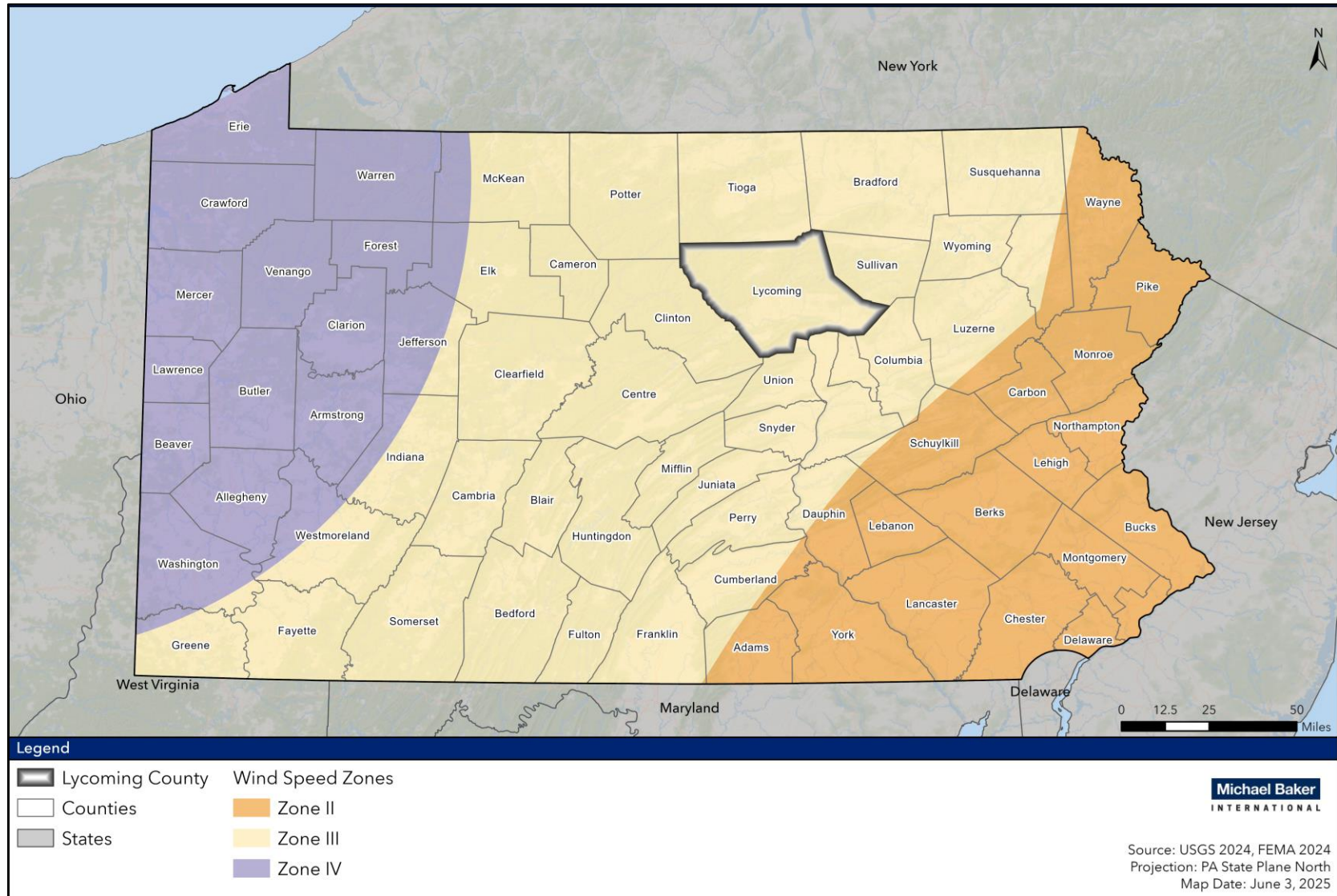
Figure 4.3.11-1 Map showing wind zones to guide design standards and shelter construction.
